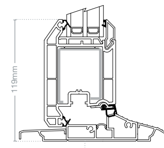
Low threshold assembly EWS 7545A and EWS 7546A
